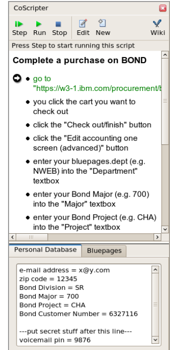
Figure 3: CoScripter sidebar (appears on left side of Firefox browser) with a script and data in the personal database.
